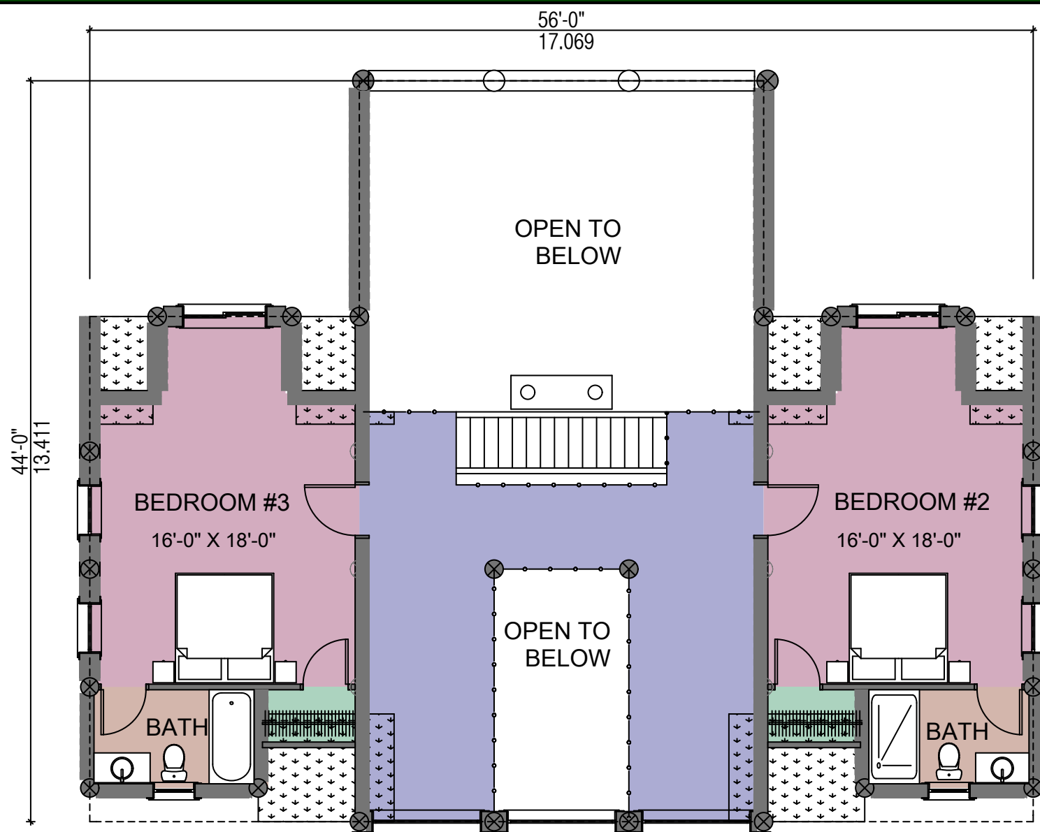
SECOND FLOOR PLAN AREA: 1128 SQ. FT. 105 SQ.M.
